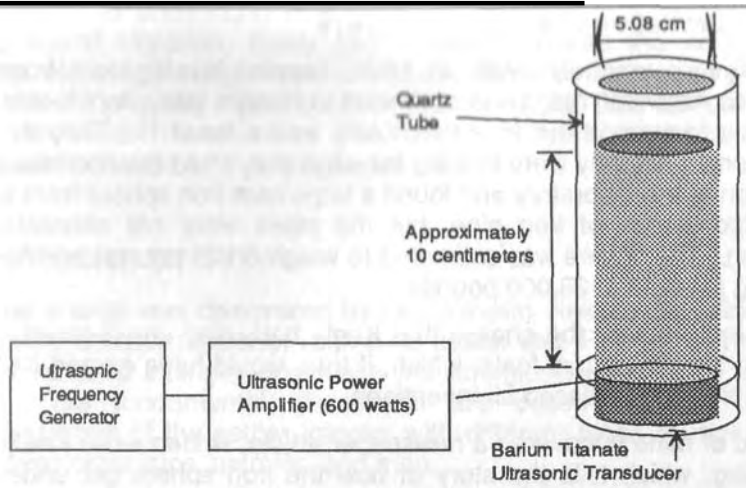
Figure 2.2.3.1-1 Modern Duplication of the Aetheralization of Water
