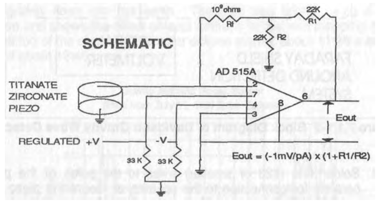
Figure 7.1.1-3 Schematic of Davidson Gravity Wave Detector
