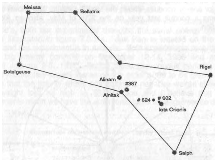
Figure 7.4.2-1. Orion Constellation
