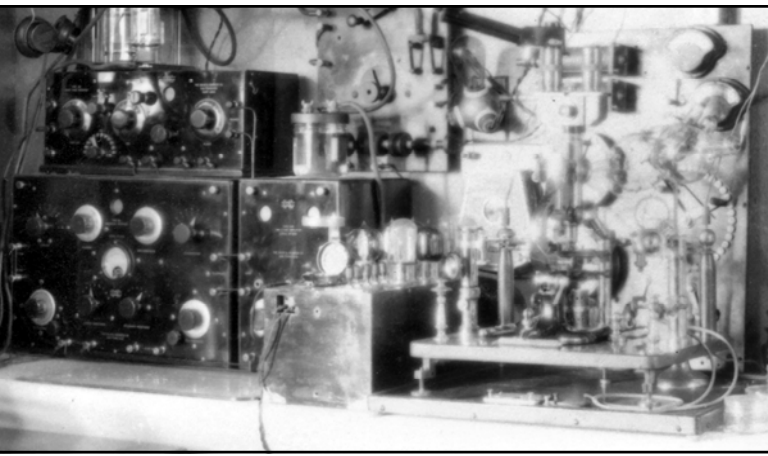
Kennedy Model 110, 281 and 525 Audio Amplifier Set Up In Rife's Lab For Doing M.O.R Work
