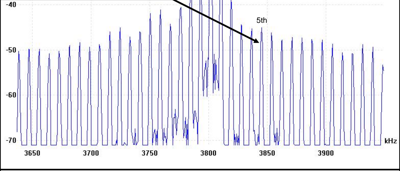
Philip Hoyland's Beam Ray Clinical instrument 3.8 Megahertz spectrum analysis of sideband harmonic frequencies.
