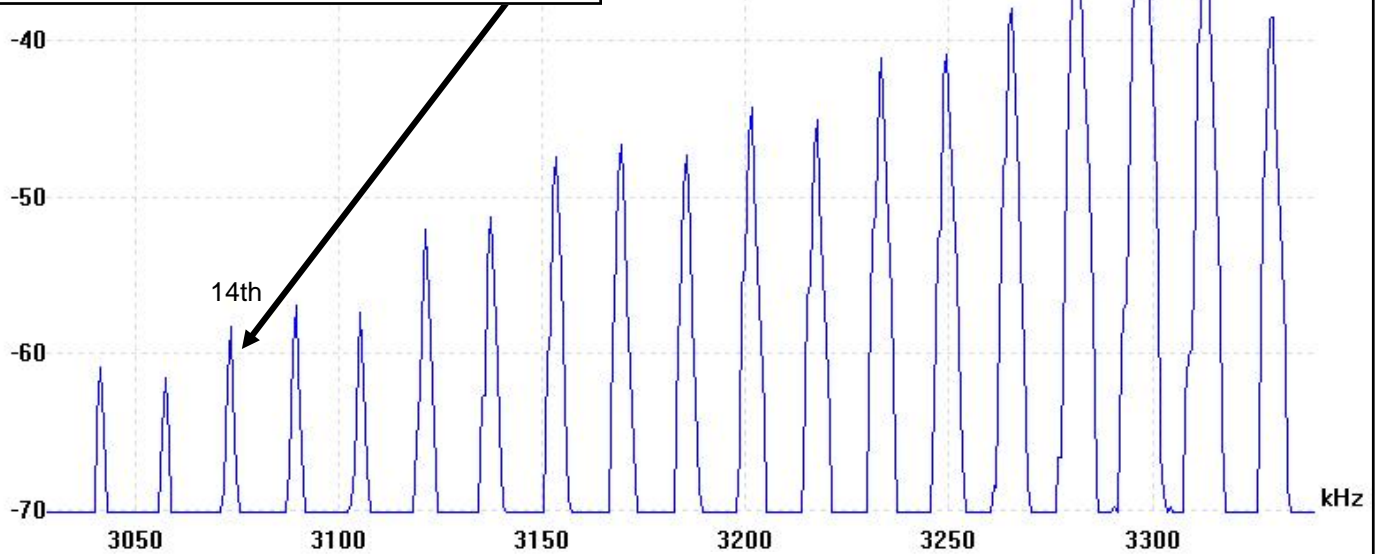
Scoon's Beam Ray Clinical instrument 3.3 Megahertz spectrum analysis of sideband harmonic frequencies.
