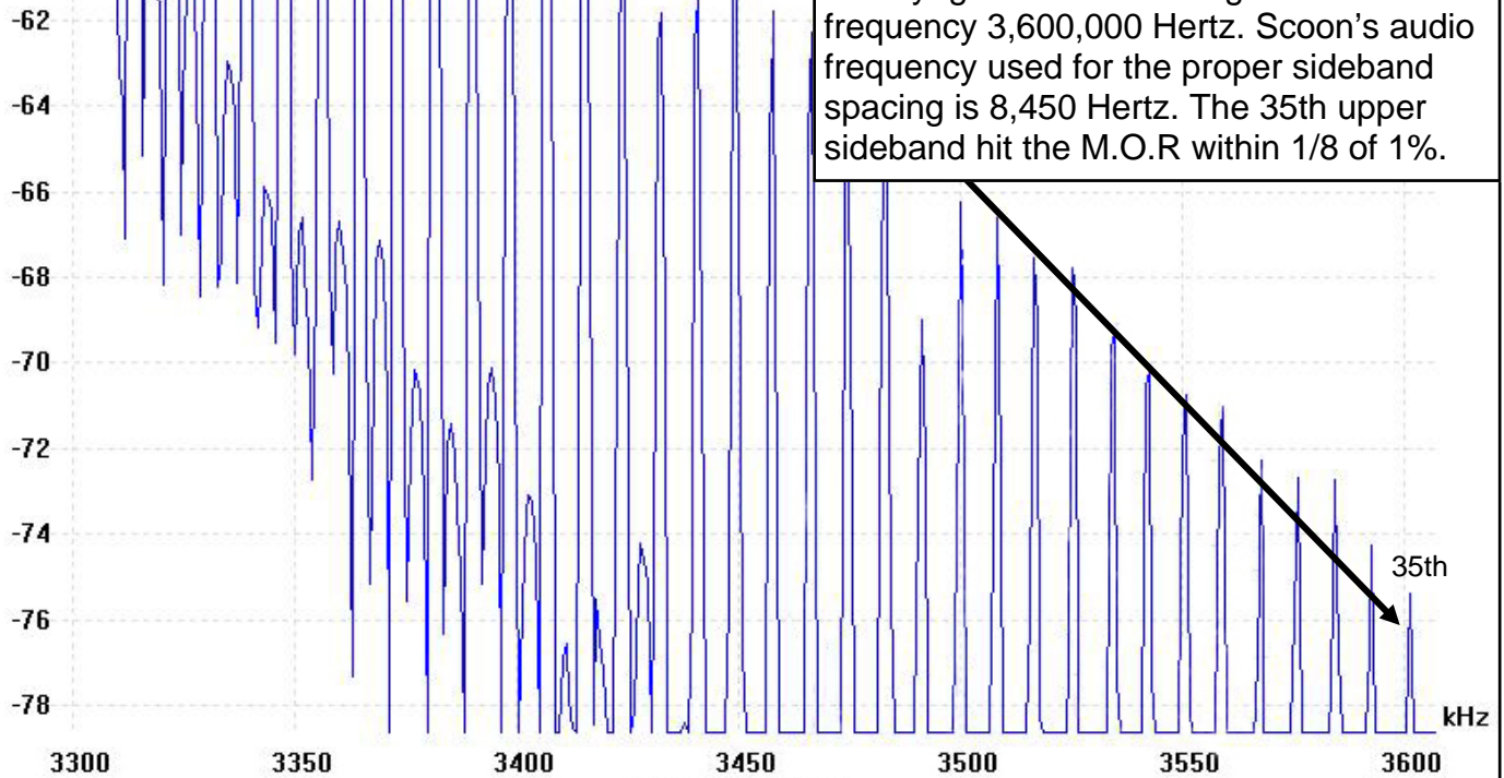
Scoon's Beam Ray Clinical replica instrument 3.3 Megahertz spectrum analysis of sideband harmonic frequencies.
