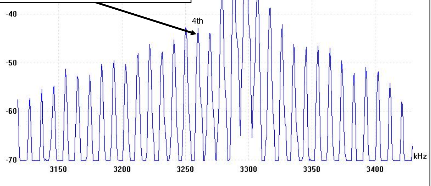
Scoon's Beam Ray Clinical replica instrument 3.3 Megahertz spectrum analysis of sideband harmonic frequencies.
