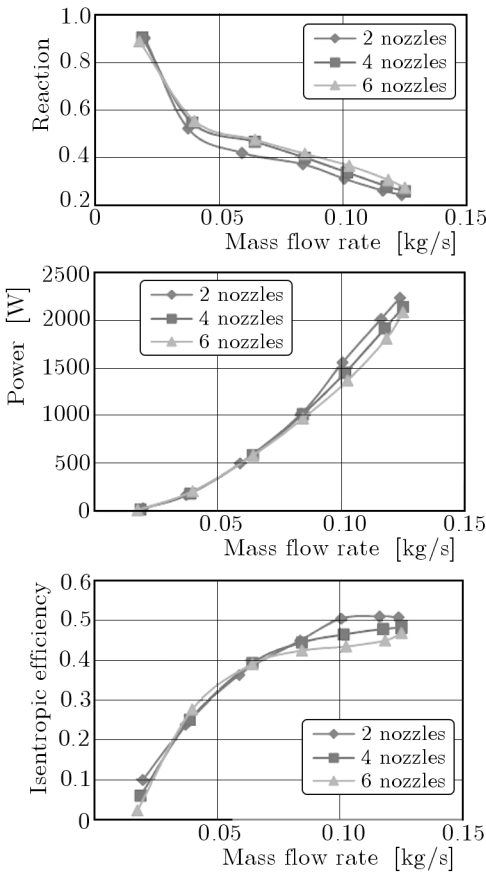
Fig. 12. Work characteristics for the model with a disk diameter 300 mm as a function of flow rate; the system supplied from two, four and six nozzles
