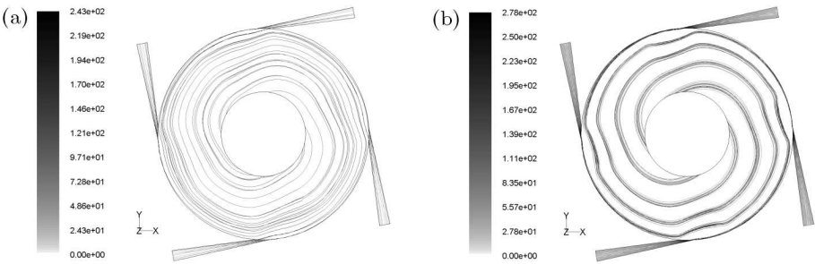
Fig. 7. Pathlines distinguished by the velocity magnitude at nominal load, disk diameter 100 mm, inlet angle 10^\circ ; (a) 18 000 rpm, (b) 9 000 rpm
