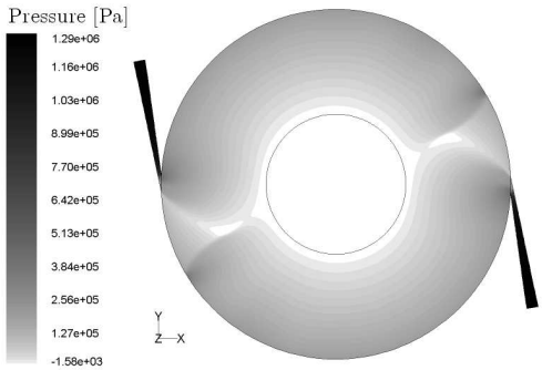
Fig. 9. Contours of static pressure; 2 supply nozzles, disk diameter 300 mm, inlet angle 10^\circ ; rotational speed 9 000 rpm
