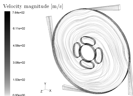
Fig. 16. Full model calculations. Pathlines distinguished by the velocity magnitude in the symmetry plane between the disks
