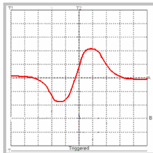
SHORT-CIRCUITED COIL
