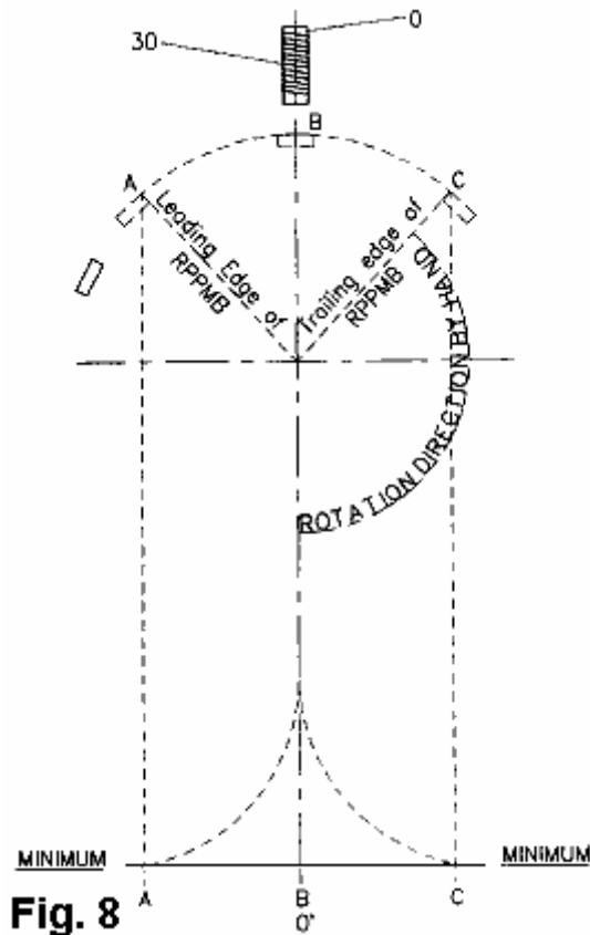
Fig.8 shows a schematic diagram of variation of natural magnetic attraction versus angular displacement of a rotor having a single permanent magnet and a stator having a single energizing coil, in accordance with a second embodiment of the present invention;
