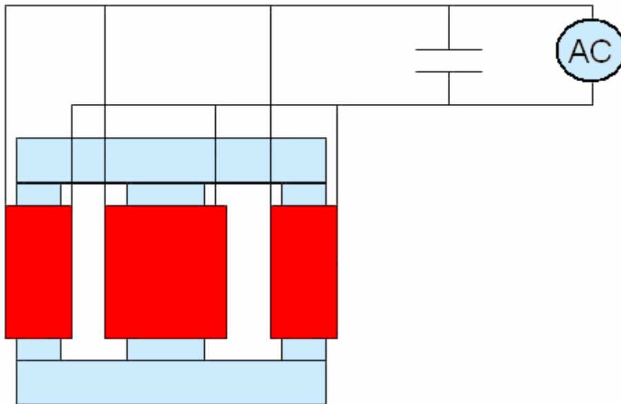
Figure 2. C-I and E-I resonant setup.
