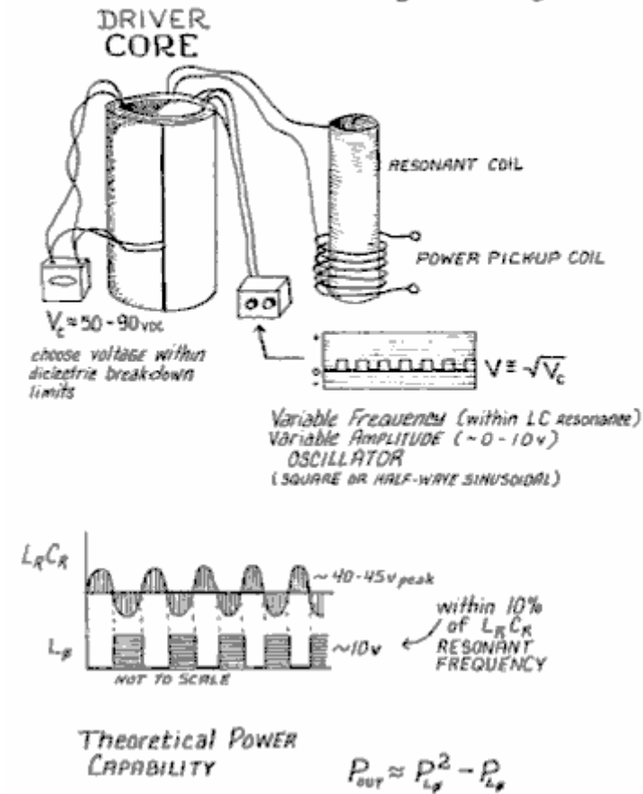
Fig.1 shows the general layout of the entire E-Stress Power System. This diagram illustrates the driver core and the variable frequency oscillator which determines the tank circuit resonance. Fig.1 also shows the DC power source of around 50 to 90 volts, which initially charges the "core" capacitor CDI / CDE . Also shown in this diagram is the resonant coil and power output or "pickup" coil.
