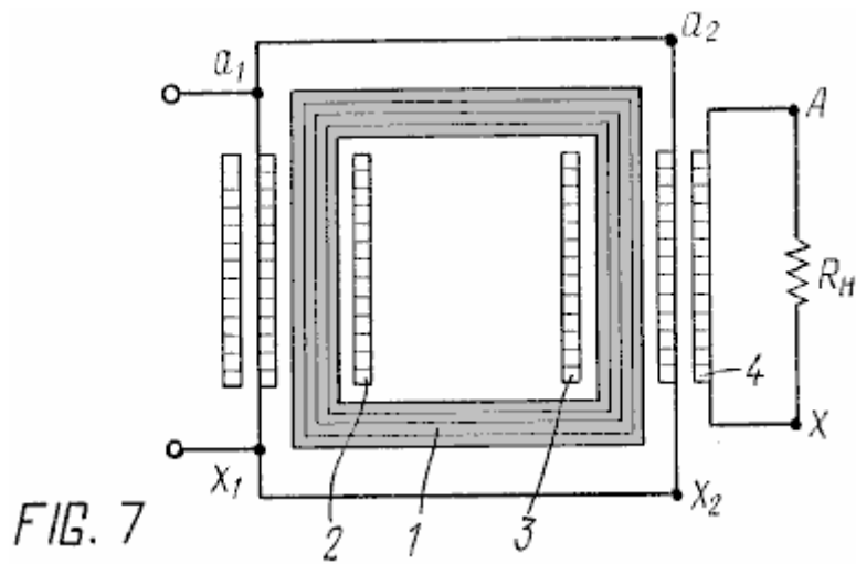
Fig.7 shows one of the embodiments of the transformer in accordance with the invention (circuit);
