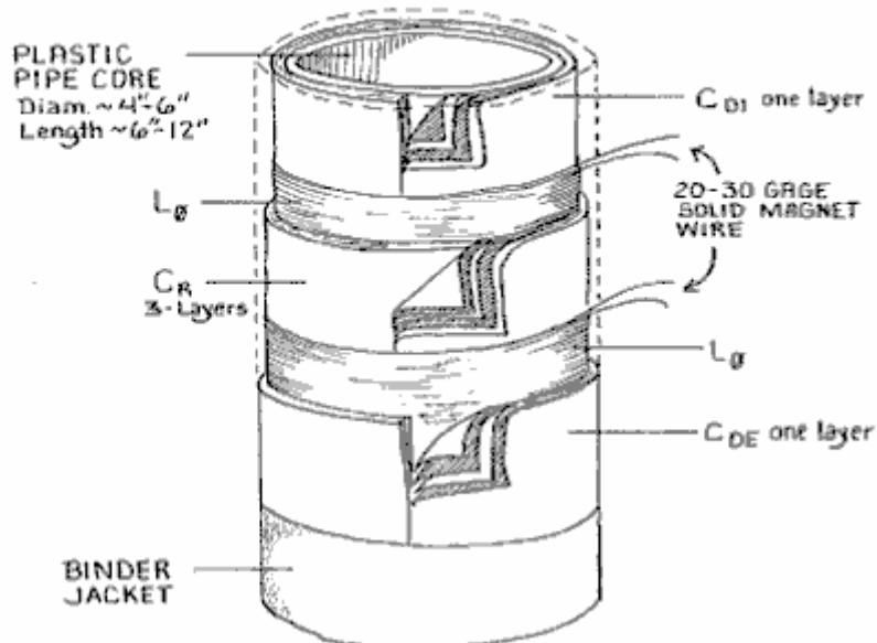
Fig.2 shows the "driver core" in a cutaway, perspective diagram. The PVC plastic "core" material can be a 6 inch (150 mm) diameter foot long (300 mm) piece of PVC pipe in this scaled-down model system. In this diagram, please note the inner and outer one-layer capacitor capacitors CDE and CDI . Also note that the middle capacitor
