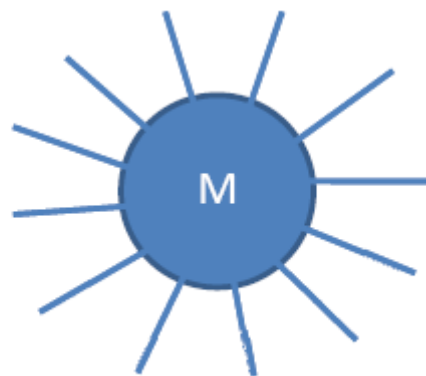
Fig.14 GRAVITATIONAL FIELD
