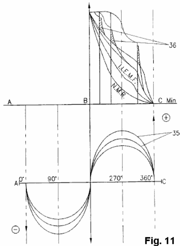
Fig.11 shows a further graphical representation of induced induction electro-magnetic force versus angular displacement of the permanent magnet in accordance with the second embodiment of the present invention.
