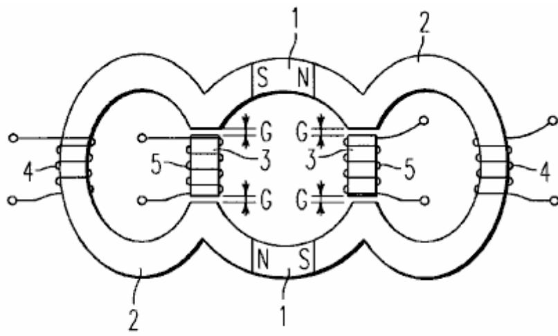
Fig.5 is a first embodiment of the static magnet dynamo involved in this invention.
