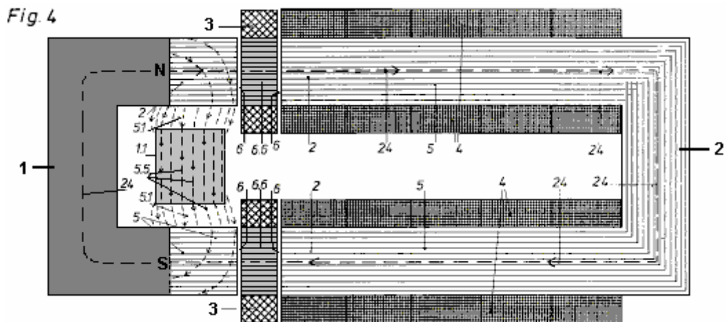
Fig.4 shows an embodiment of the above design which uses a U-shaped permanent magnet 1 and a U-shaped generator core 2 which has its two ends facing towards the poles of the permanent magnet 1. Wound around two narrow air gaps 6 and its own narrow core, is a magnetic flux modification coil 6.6.
