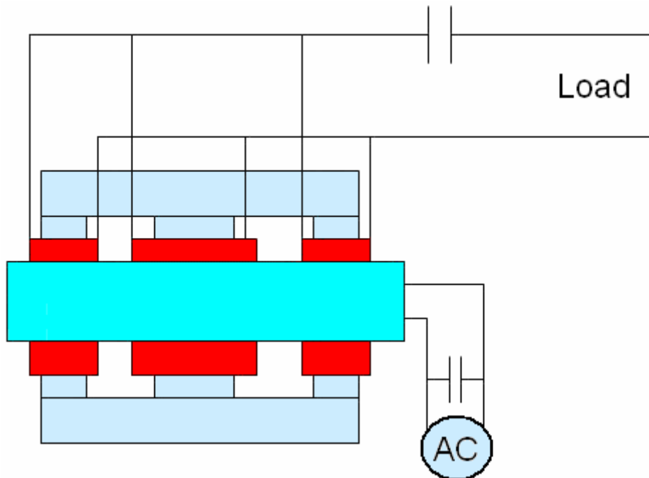
Figure 3. C-I and E-I with primary on top.
