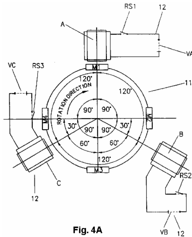
As shown in Fig.4A according to the first embodiment of the invention a system is provided consisting of a rotor 11 having four permanent magnets M1, M2, M3, M4 which are evenly spaced at 90° with respect to each other.
