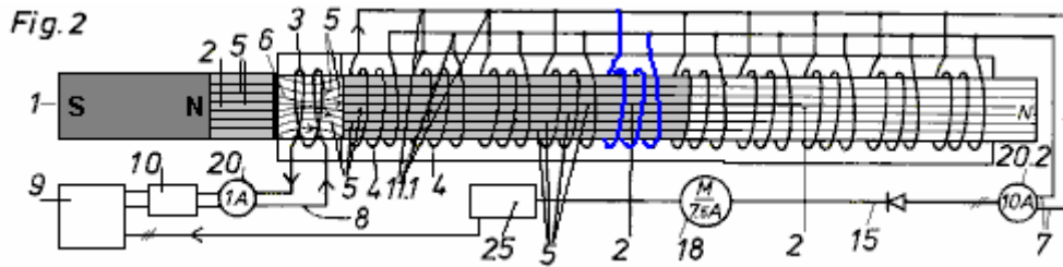
Fig.2 illustrates that on the generator core 2 several induction windings 4 are wound, which correspond to the number of turns with same wire diameter as used in the magnetic flux modification coil 3.
