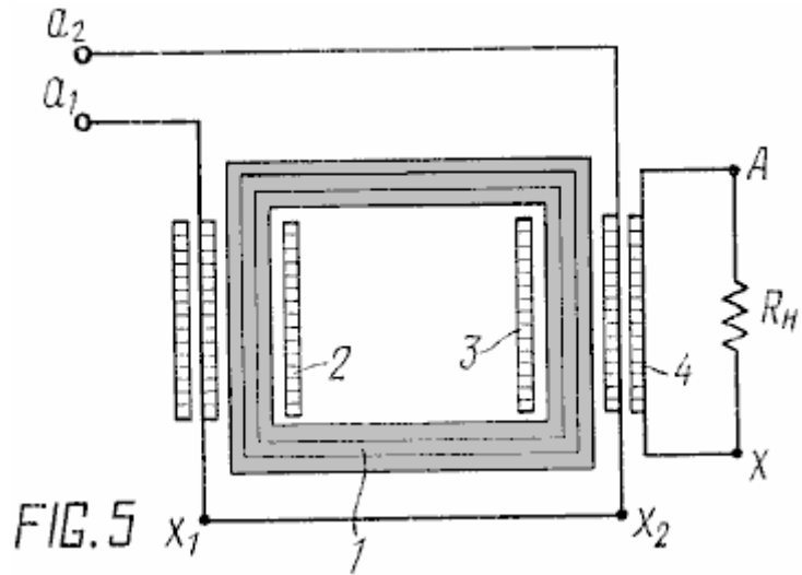
Fig.5 shows one more embodiment of the transformer in accordance with the invention (circuit);
