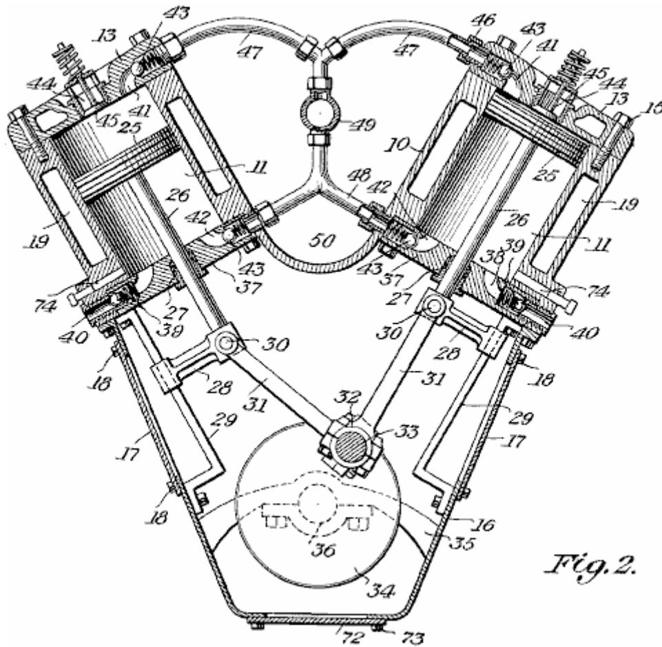
Fig.2 is a vertical transverse cross-section view through the compressor part of the engine.
