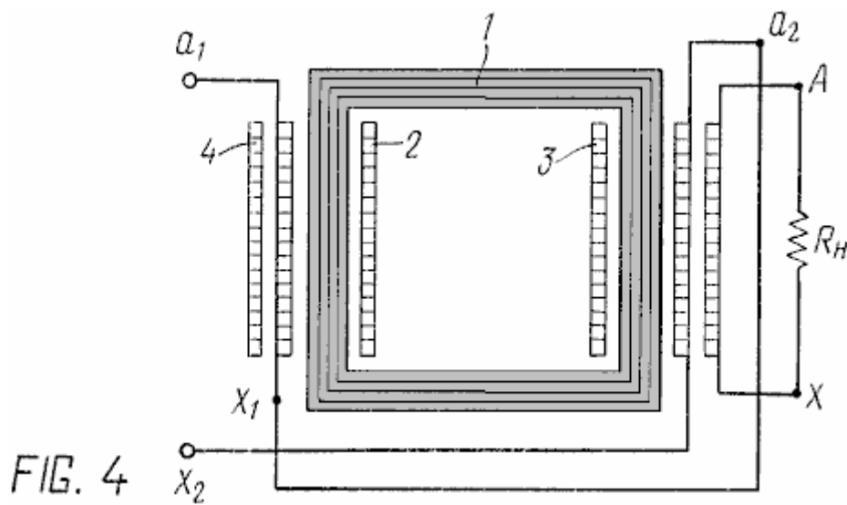
FIG.4 shows one more embodiment of the transformer in accordance with the invention (circuit);
