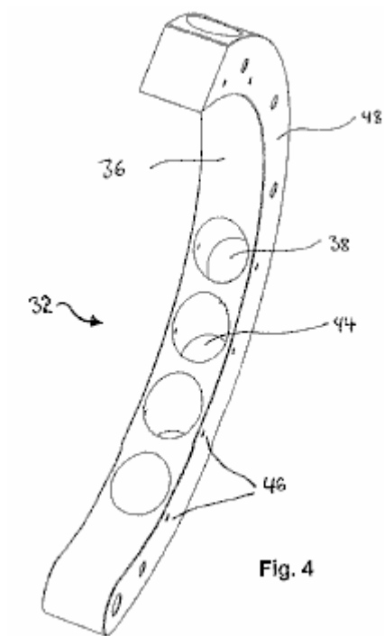
Fig.4 is a perspective view showing a right arm of a stator
