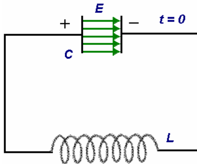
Oscillating circuit. Charged capacitor (electric field) discharges, current carried through insulated wire to charge coil (magnetic field) which discharges, charging capacitor. Oscillating electric and magnetic fields yield electromagnetic waves.
